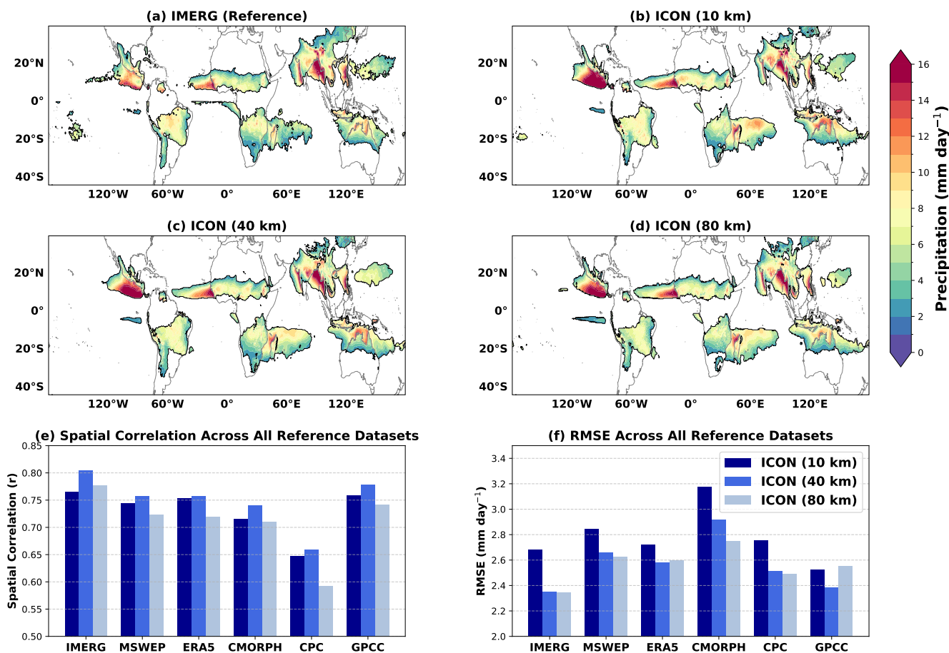
Figure 1. Global monsoon domains (contours), defined by regions where local summer minus winter precipitation difference is > 2 mm/day and summer precipitation contribution is \geq 55\% of annual total. The shaded regions show the annual range of precipitation (local summer minus winter) in (a) IMERG observations and (b-d) ICON simulations at 10 km, 40 km, and 80 km grid spacing. (e) Spatial correlation and (f) RMSE of the monsoon precipitation annual range for ICON simulations against six observational datasets (2007-2016). The spatial correlation and RMSE values are statistically significant with p < 0.05 based on a two-sided Student's t-test. All the datasets are plotted and analyzed at a common grid close to ERA5 with a grid spacing of about 30 km.
