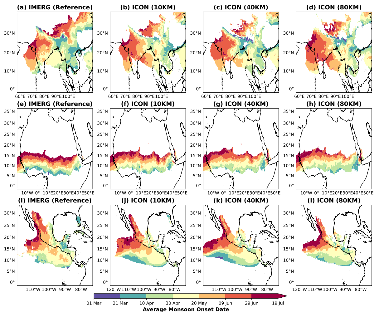
Figure 3. Spatial patterns of monsoon onset dates over the (a-d) SAsiaM, (e-h) WAFriM and the (i-l) NAmM domain in IMERG and ICON simulations. The onset of a monsoon is defined as the first day starting from March, on which pentad-mean (5-day running mean) precipitation exceeds 5 mm/day for at least three consecutive pentads. The definition of the monsoon onset is consistent across various monsoon domains to ensure the property of universal applicability.
