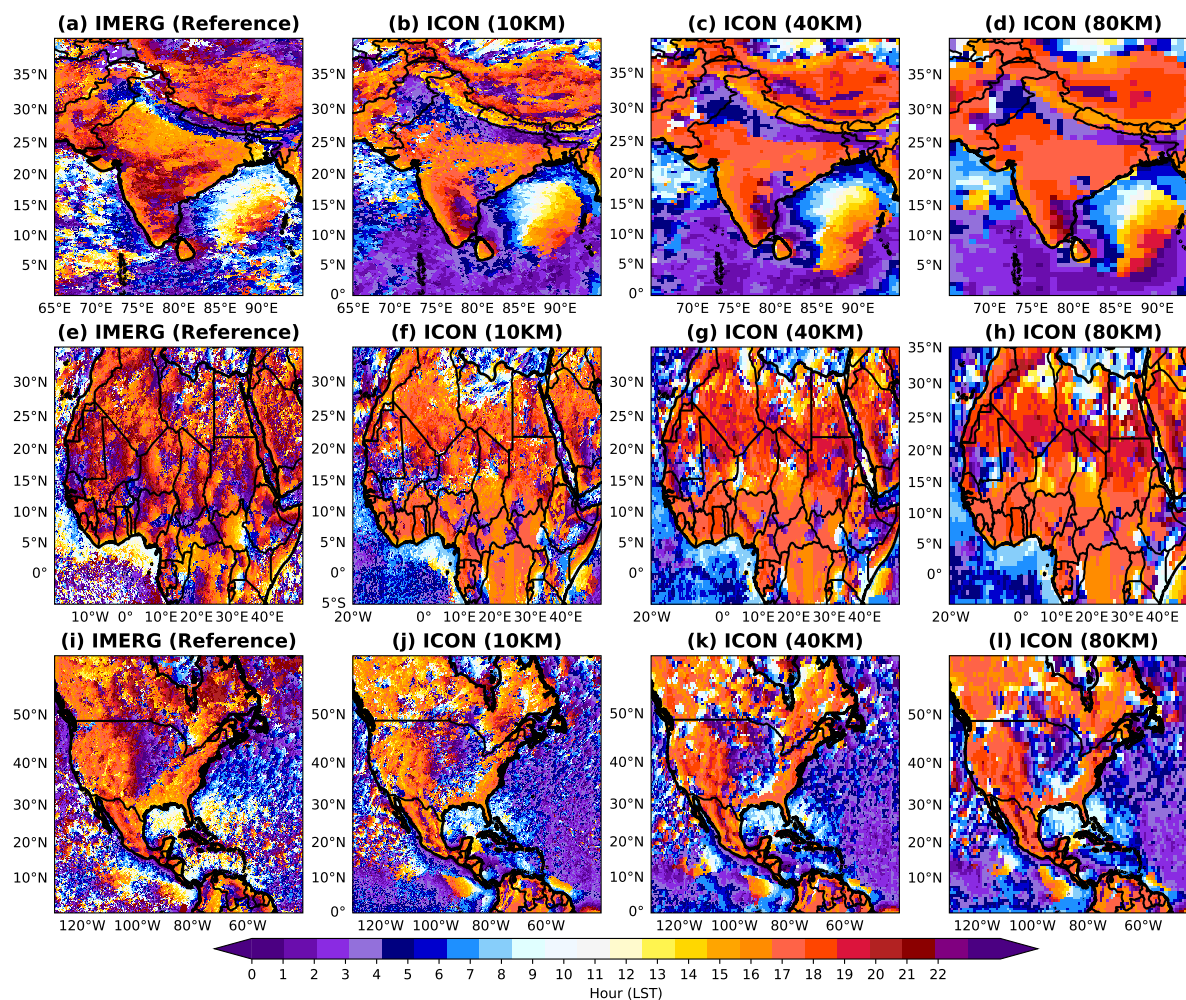
Figure 11. The local solar time (LST) at which maximum precipitation occurs on on average during the summer monsoon season (JJAS), showcasing a peak time of diurnal cycle in IMERG reference dataset and the ICON simulations over the (a-d) SAsiaM, (e-h) WAFriM, and (i-l) NAmM domain. The shading of blue/dark purple indicates a nocturnal maxima while the colors shaded from yellow/red show afternoon or late evening peak.
