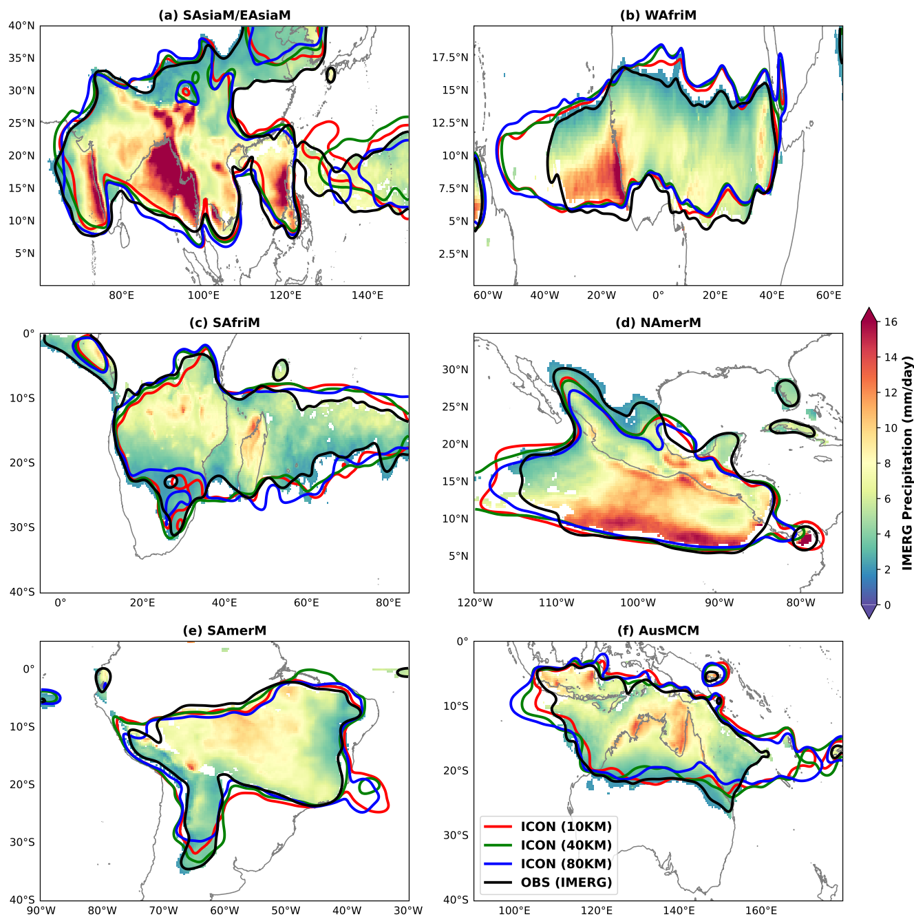
Figure 2. Regional monsoon domains (a) SAsia/EAsiaM (b) WAFriM (c) SAfriM (d) NAmM (e) SAmM (f) AusMCM detected in various ICON simulations and IMERG reference dataset defined as the regions where the local summer minus winter precipitation is > 2 mm/day and summer contribution is \geq 55\% of annual total. The black contours show monsoon domains in IMERG observational dataset, while the red, blue, green show the boundaries for 10 km, 40 km, 80 km simulations respectively. The shading shows the total precipitation in mm/day (local summer) from IMERG reference dataset. Contours are Gaussian-smoothed ( \sigma=3 ) for clarity.
